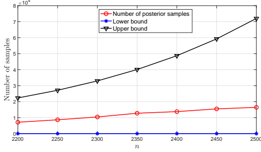
Figure 1: Average number of posterior samples versus n .
