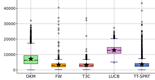
Figure 6: Sample complexity (Gaussian): \mu = [1, 0.85, 0.8, 0.7] , \delta = 0.1
