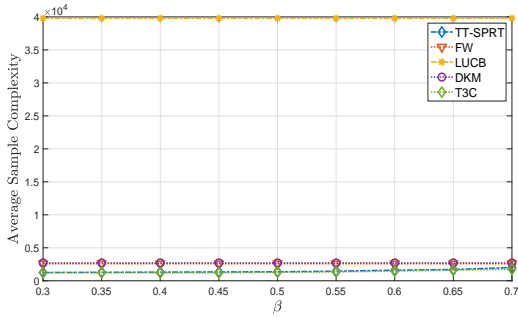
Figure 7: Sensitivity to \beta : (Bernoulli)
