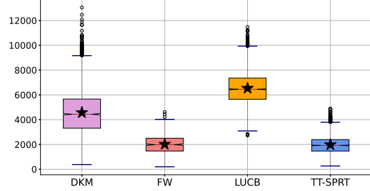
Figure 10: Sample complexity (Exponential)
