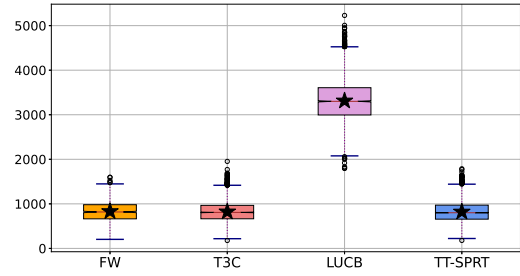
Figure 4: Sample complexity (Gaussian): \mu = [5, 4.5, 1, 1, 1] , \delta = 10^{-15}
