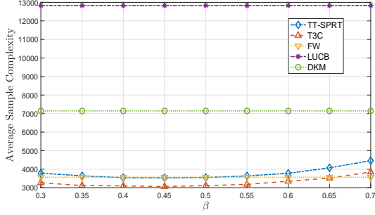
Figure 5: Sensitivity to \beta (Gaussian): \mu = [1, 0.85, 0.8, 0.7] , \delta = 0.1
