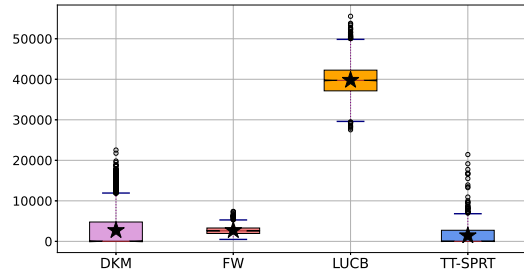
Figure 8: Sample complexity (Bernoulli)
