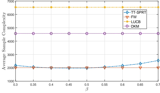
Figure 9: Sensitivity to \beta : (Exponential)
