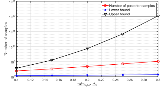
Figure 2: Average number of posterior samples versus gaps.
