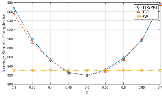
Figure 3: Sensitivity to \beta (Gaussian): \mu = [5, 4.5, 1, 1, 1] , \delta = 10^{-15}
