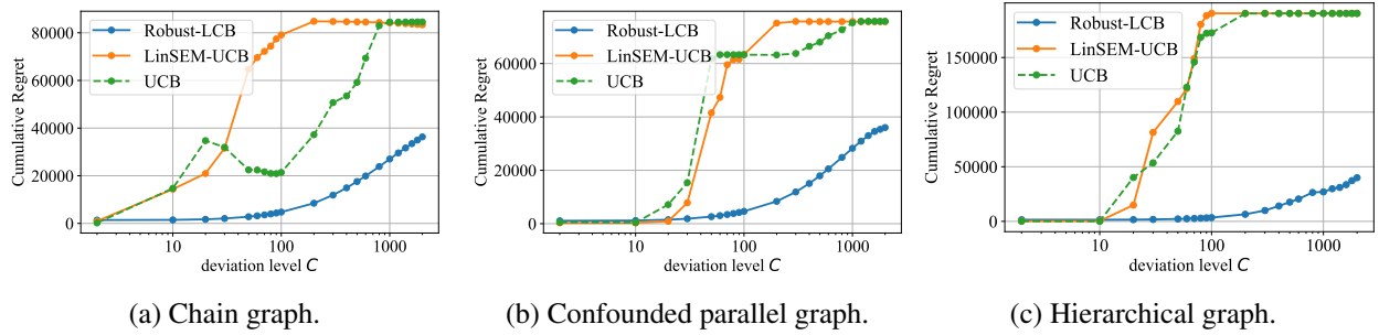
Figure 7: Cumulative regret at T = 40000 for different deviation levels C .
