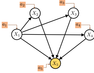
Figure 3: Confounded parallel graph N = 5 .
