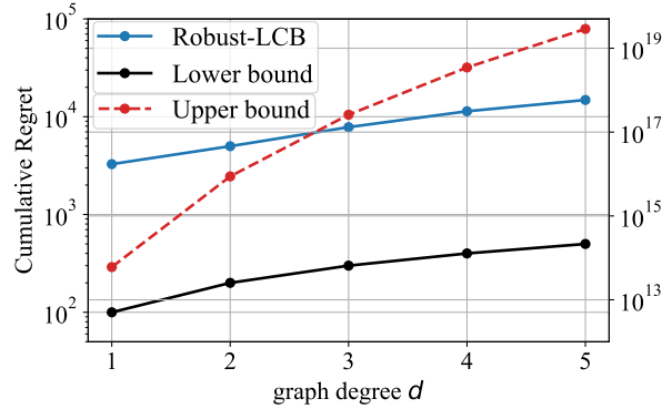
Figure 5: Cumulative regret of Robust-LCB with different graph degree d and L = 2 , N = Ld + 1 .
