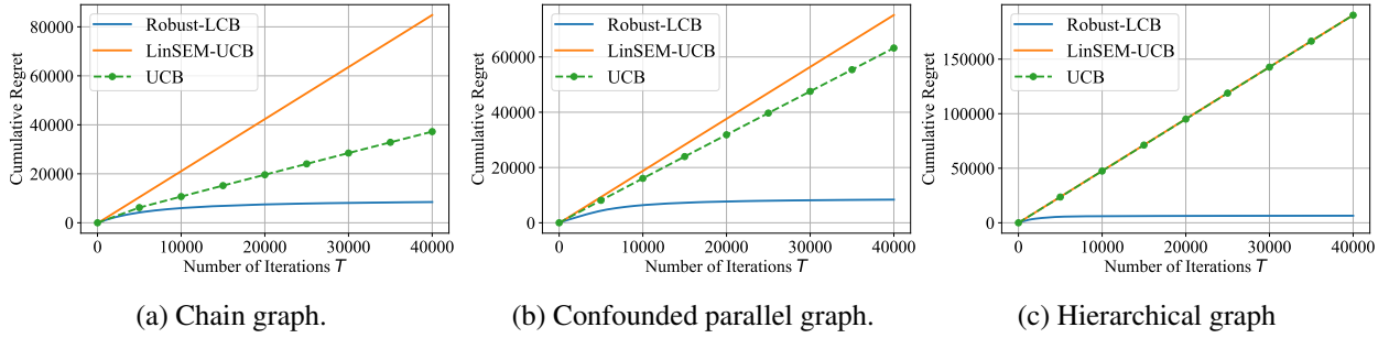
Figure 6: Cumulative regret when C = \sqrt{T} for different algorithms.
