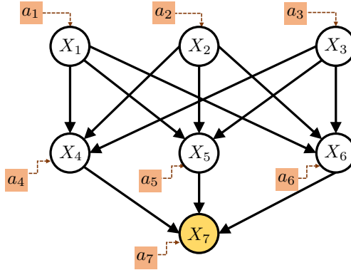
Figure 1: Example of the hierarchical graph with graph degree d = 3 and length L = 2 .
